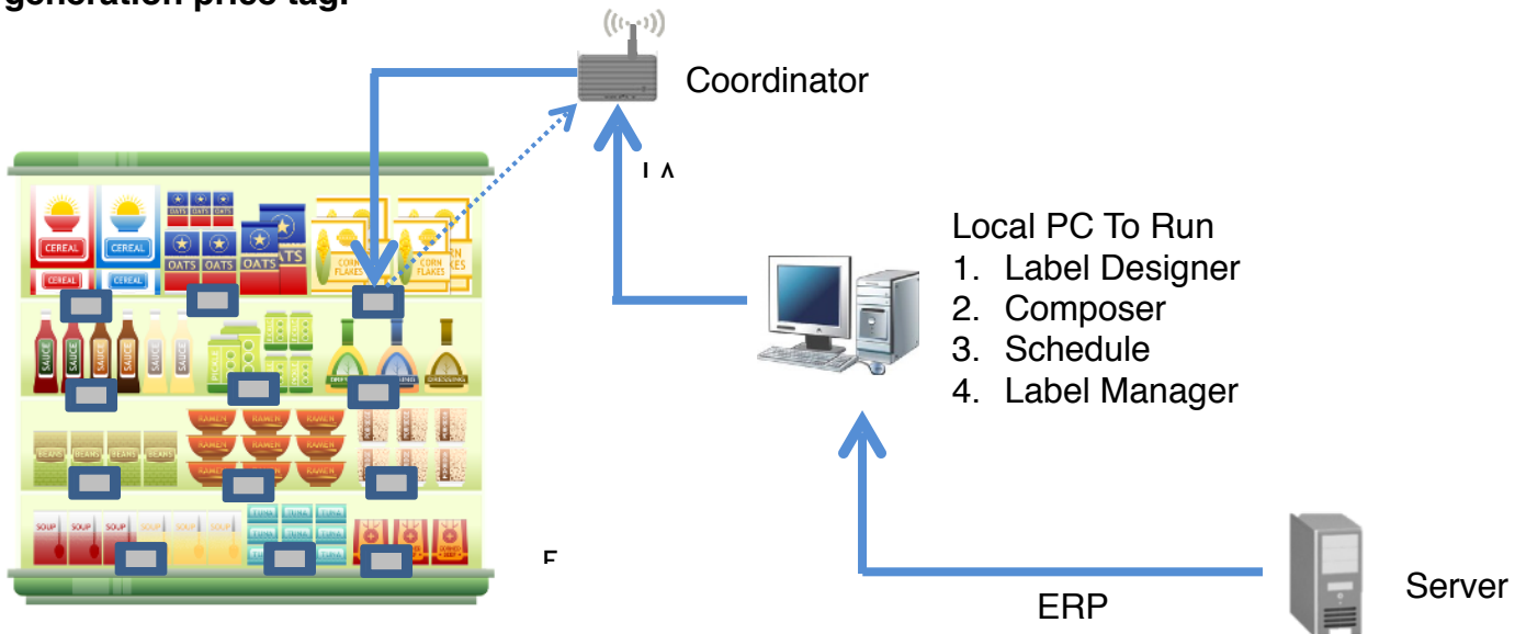
Application Architecture
